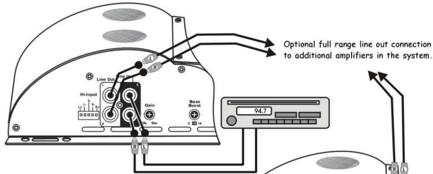
TWO CHANNEL SIGNAL CONNECTIONS
